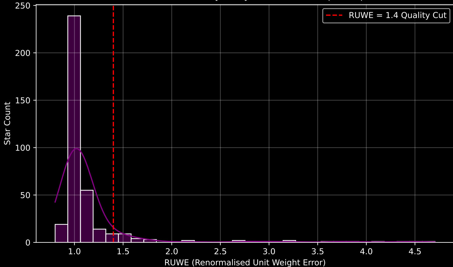
GAPOGEE DR17 Field [GD1-5] RUWE Distribution (n= 367)
