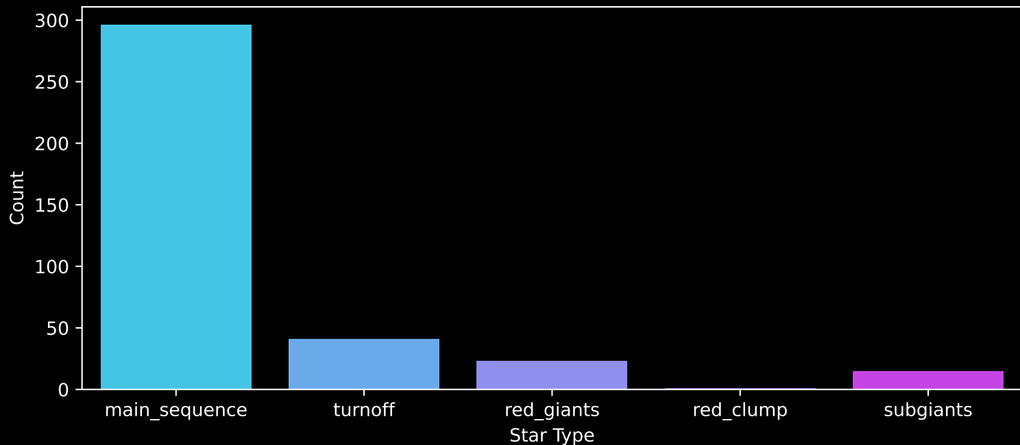
APOGEE DR17 Field: [GD1-5] Count plot of Star Type
