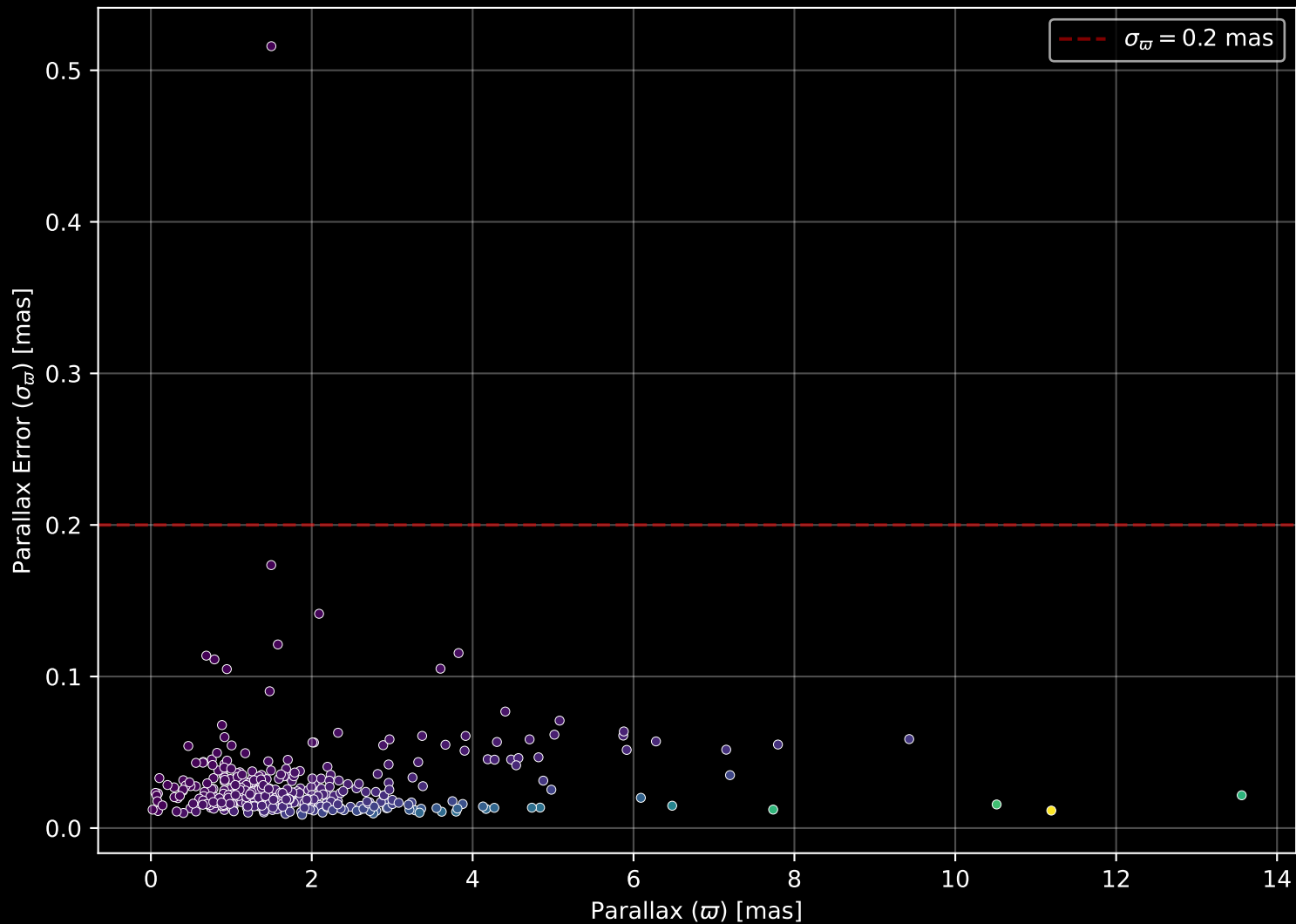
APOGEE DR17 Field: [GD1-5] Parallax Quality (n= 376)
