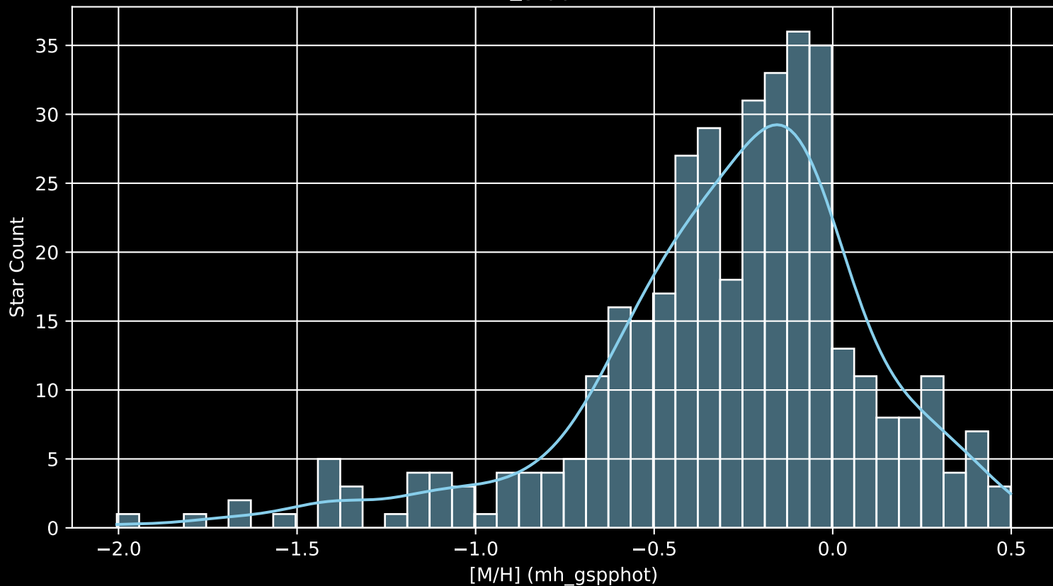
APOGEE DR17 Field: [GD1-5 [M/H] (mh_gspphot) (n= 376)
