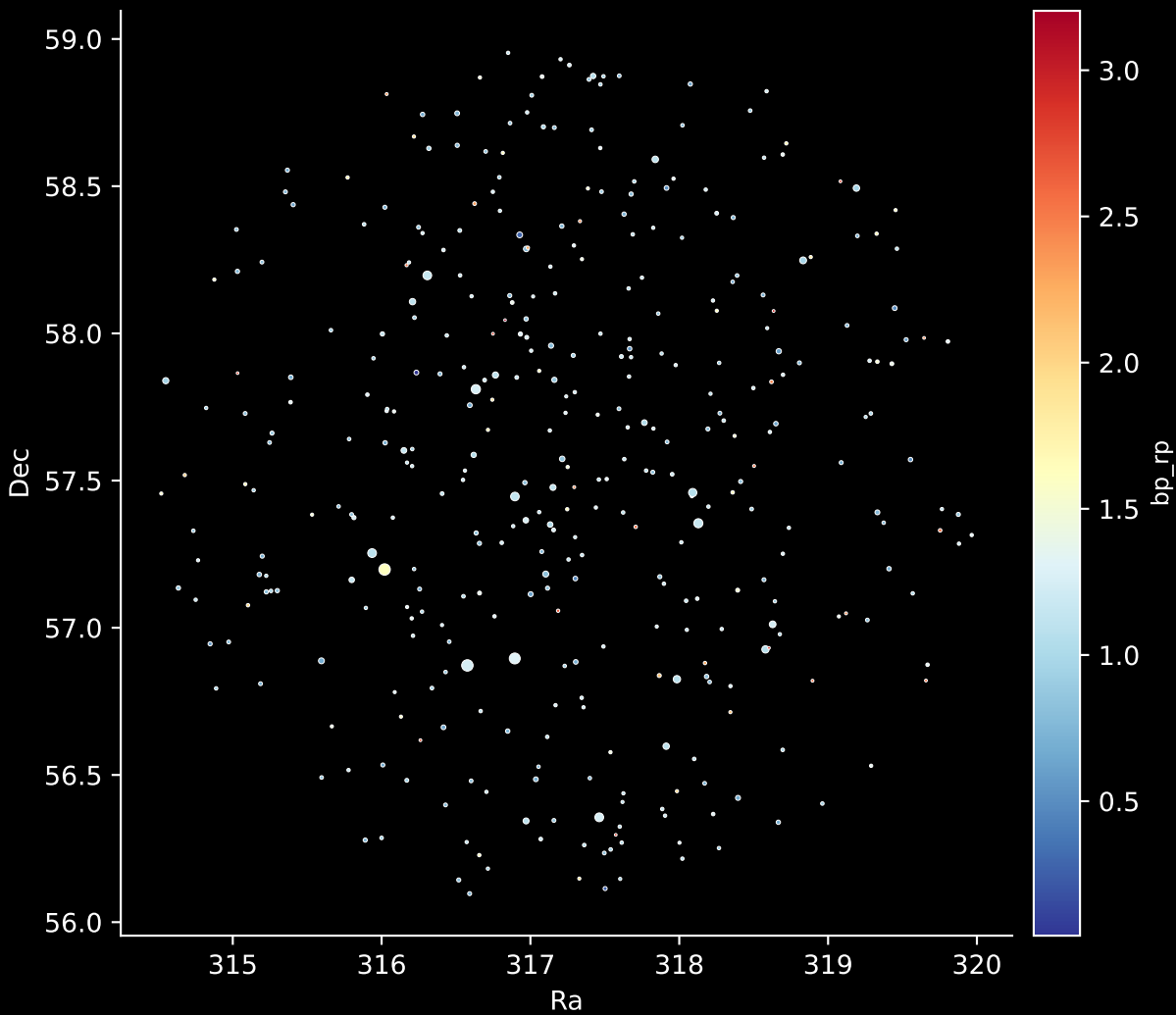
APOGEE DR17 Field: [GD1-5] Stars: 376
