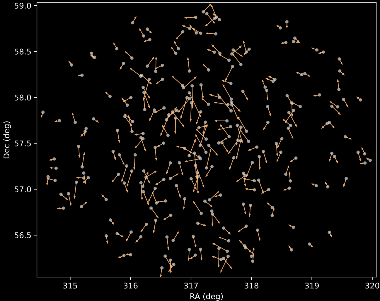
APOGEE DR17 Cluster 3 Proper Motion Vectors (n=262)
