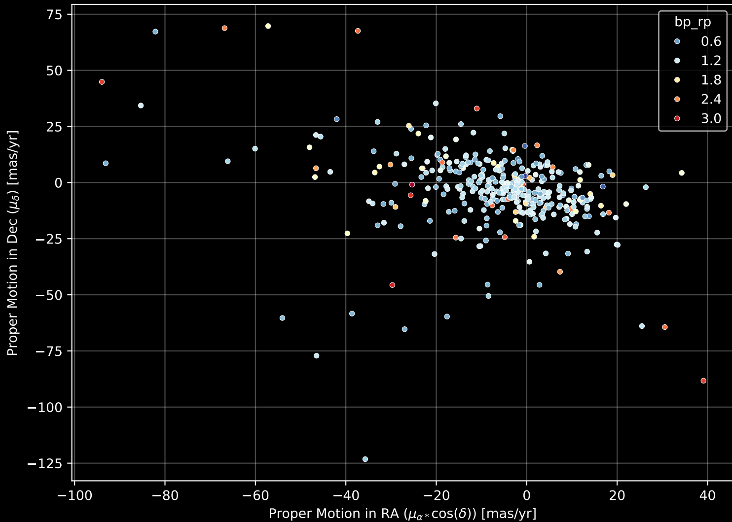
APOGEE DR17 Field: [GD1-5] Proper Motion Diagram (n= 376)
